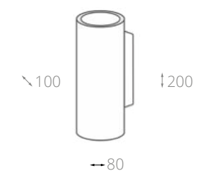
▲ C191-WL-02-W LED 2 × GU10 5W 220-240 V, IP20 200 × 80 × 100 мм
