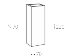
◀ C190-WL-02-W LED 2 × G9 5W 220-240 V, IP20 220 × 70 × 70 мм
